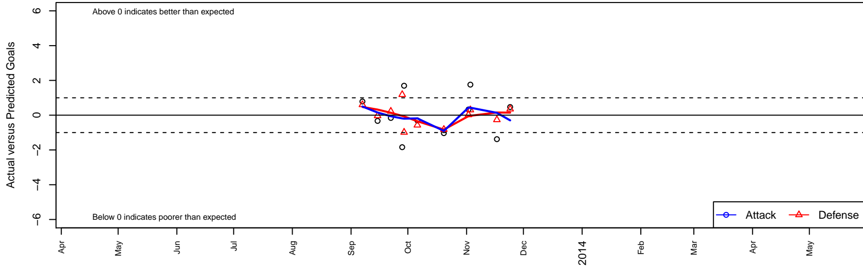
CZ Elite B94 Dots are actual minus expected GF (blue circles) and GA (red triangles). Blue line is smoothed change in attack strength. Red is smoothed change in defense strength.
